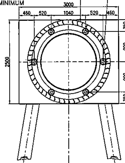
FRONT ELEVATION
