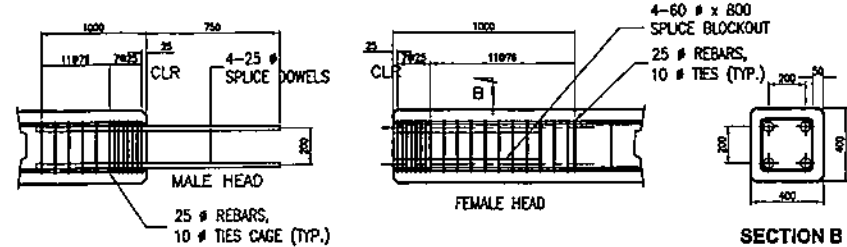
PILE SPlicing DETAIL SCALE 1:30
